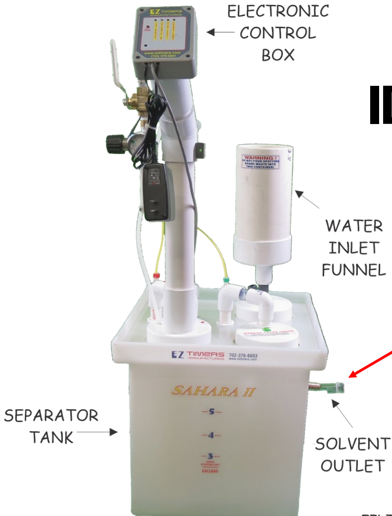
FRONT VIEW
