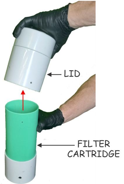
STEP 2: Remove the lid from the filter cartridge and then dump the used filter granules into your hazardous waste drum.
